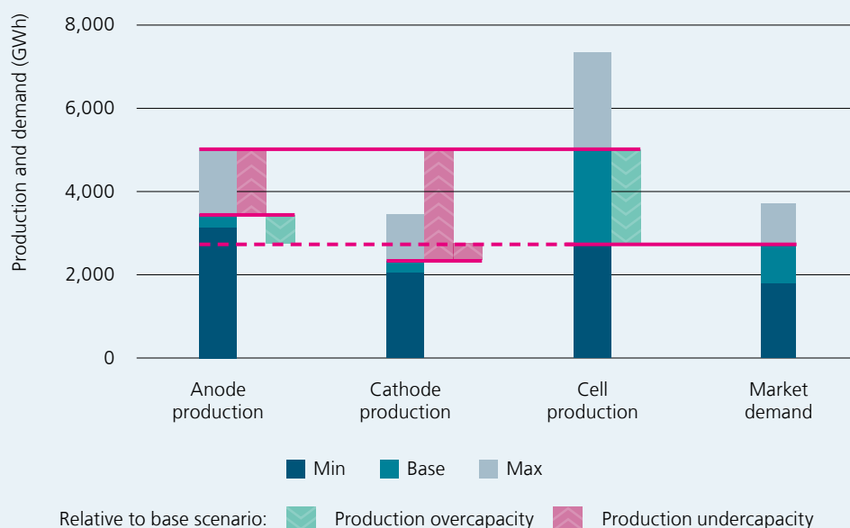
Figure 37: Comparison of global active material and cell production capacities as well as battery cell demand for 2028.
