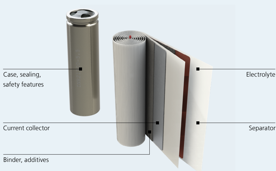
Figure 17: Components of LIB cells.
